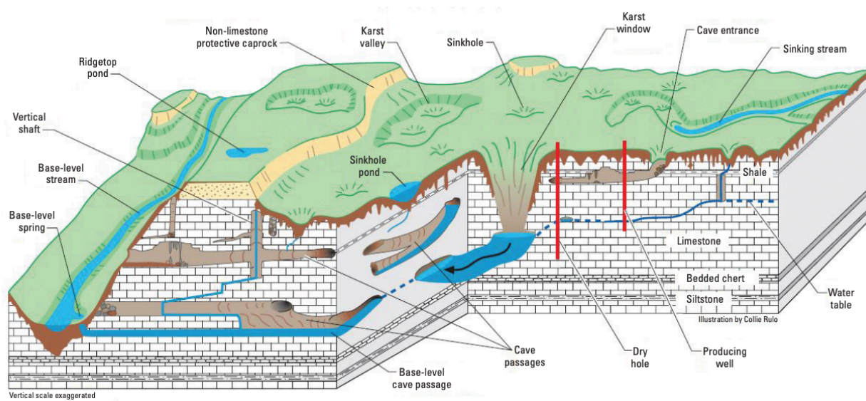
Figure 3-7 Cross section through limestone showing underground drainage, sinkholes and pinnaced bedrock. From Taylor et al. (2014).
